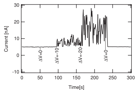
FIG. 3. Current reading versus the potential difference \Delta V between the sample holder and the last lens element before the sample holder (the distance between the two planes is \sim 5 \text{ mm} ). Note that the fluctuations in the current increase dramatically even for very small potential difference. See text for details.
